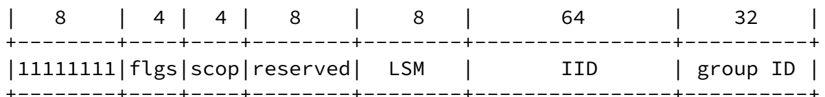
Figure 1: Link scoped multicast IPv6 address format
