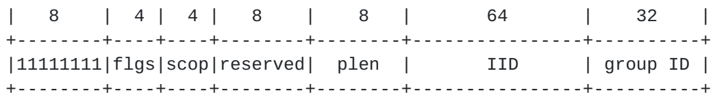
Figure 1: Link scoped multicast IPv6 address format
