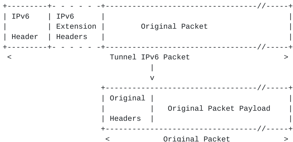
Fig.4 Decapsulating a Packet
