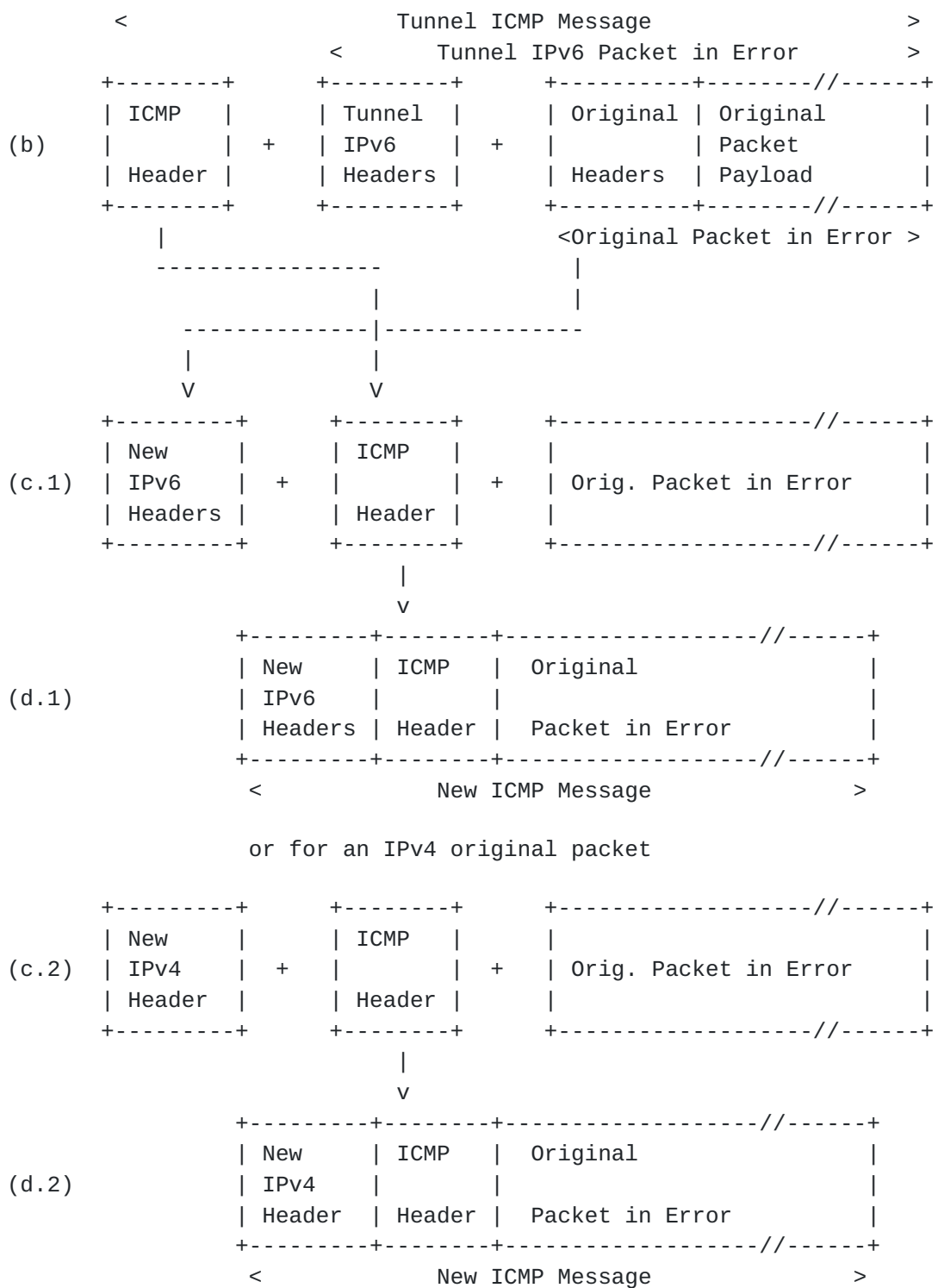
Fig.8 ICMP Error Reporting and Processing
