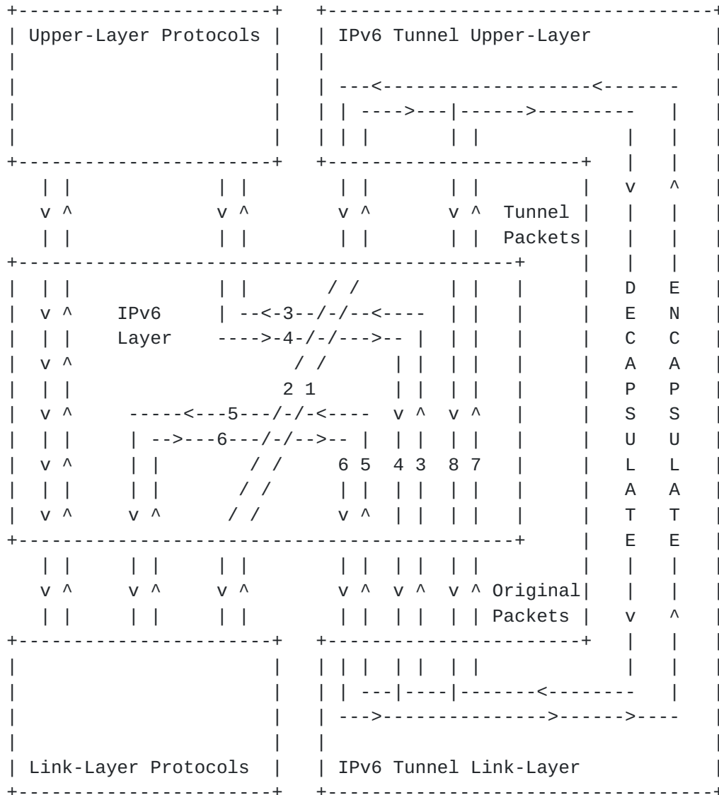
Fig.5 Packet Flow in the IPv6 Tunneling Protocol Engine on a Node
