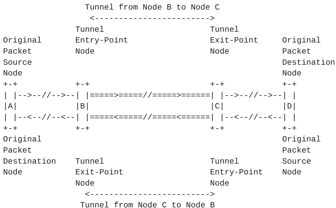
Fig.2 Bi-directional Tunneling Mechanism
