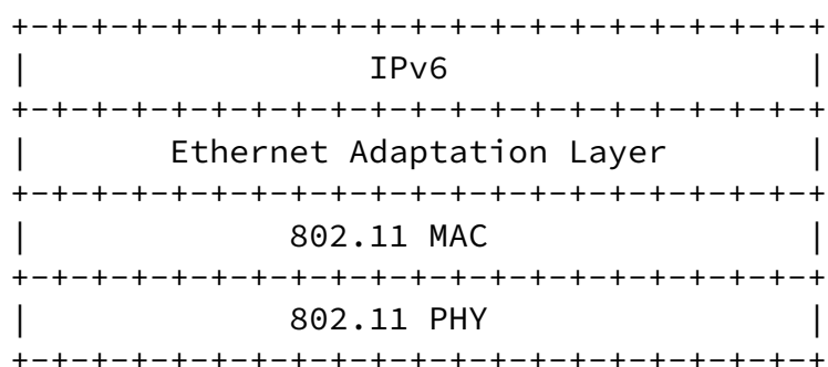
Figure 2: Ethernet Adaptation Layer stacked with other layers
