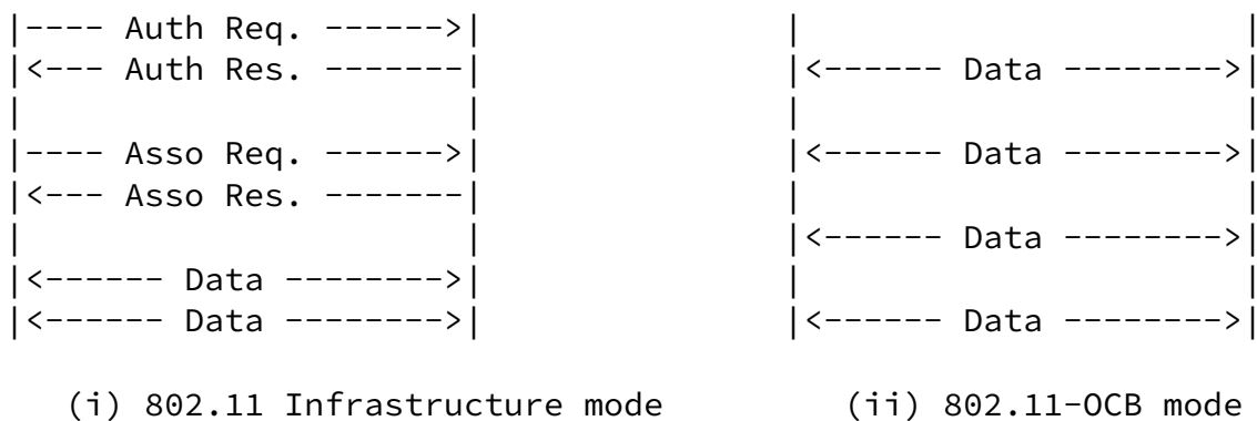
Figure 3: Difference between messages exchanged on 802.11 (left) and 802.11-OCB (right)
