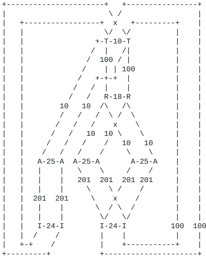
Figure 3: Explicit Routing topology
