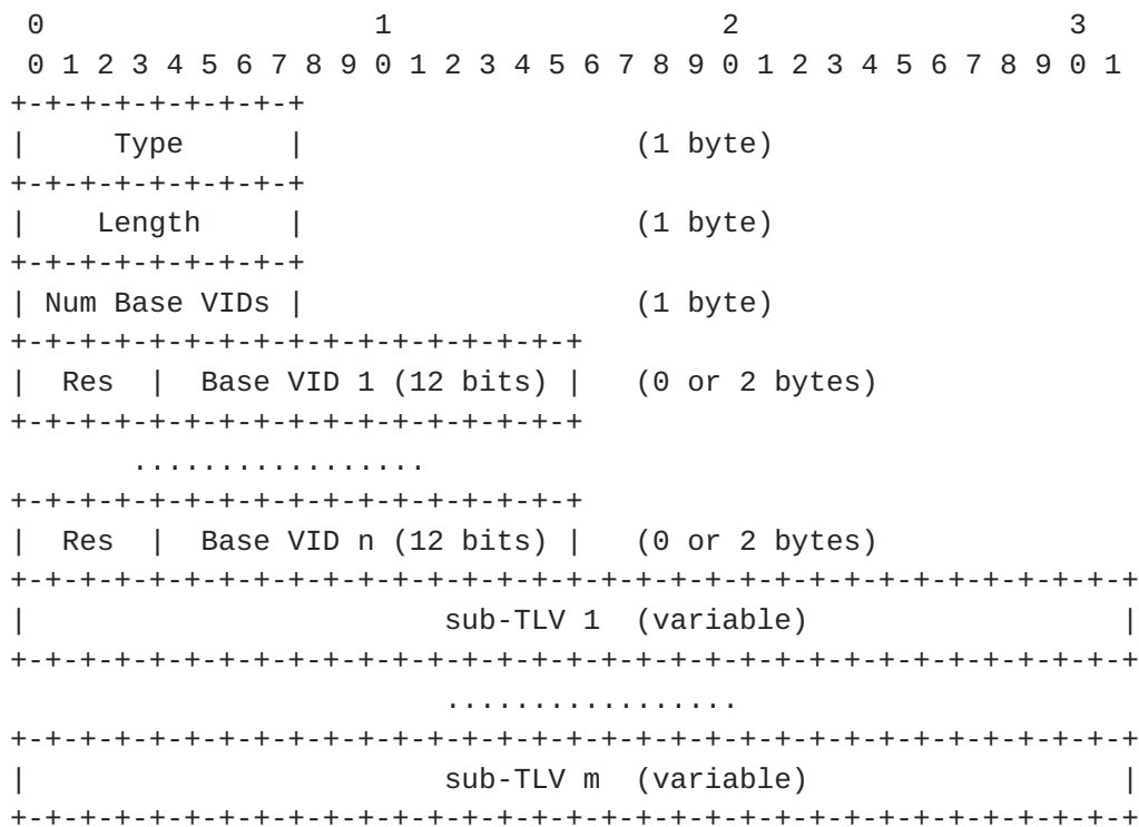
Figure 1: Topology sub-TLV
