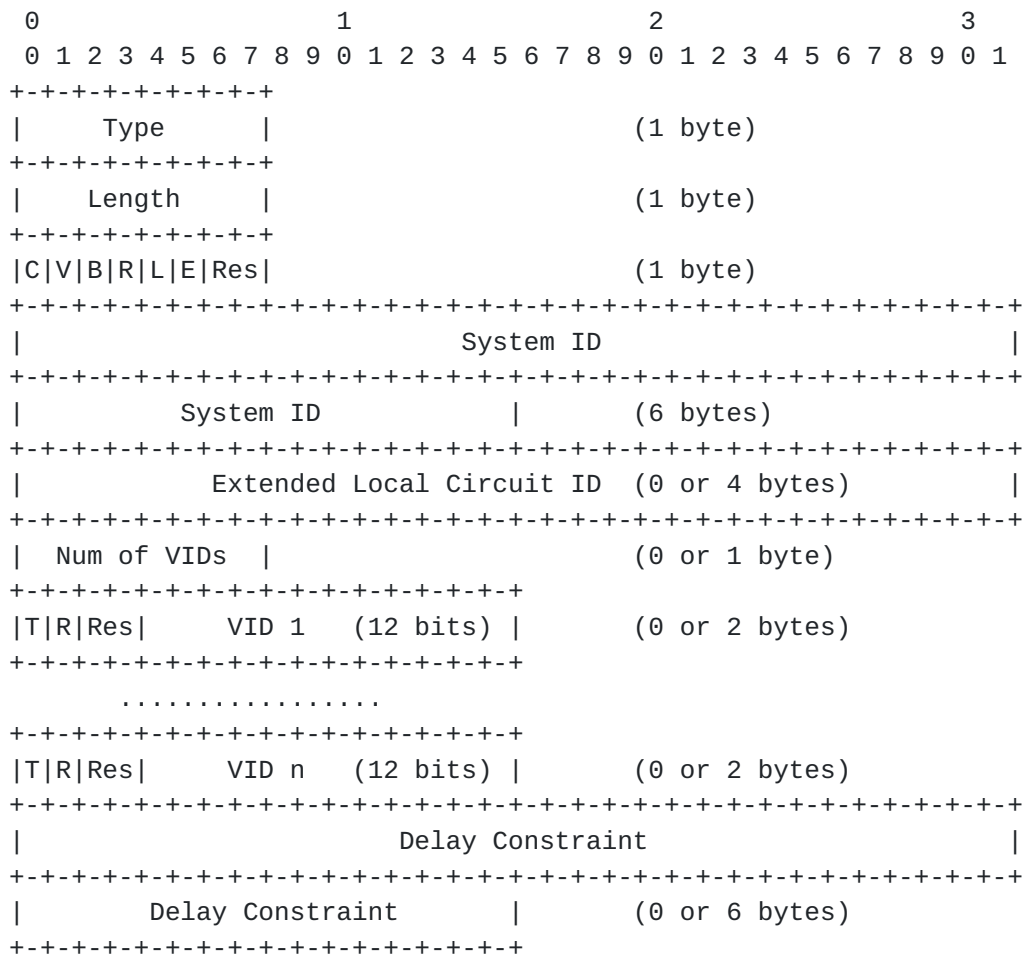
Figure 3: Hop sub-TLV
