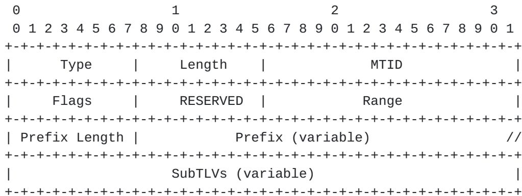
Figure 2: Multi-Topology SID/Label Binding TLV format
