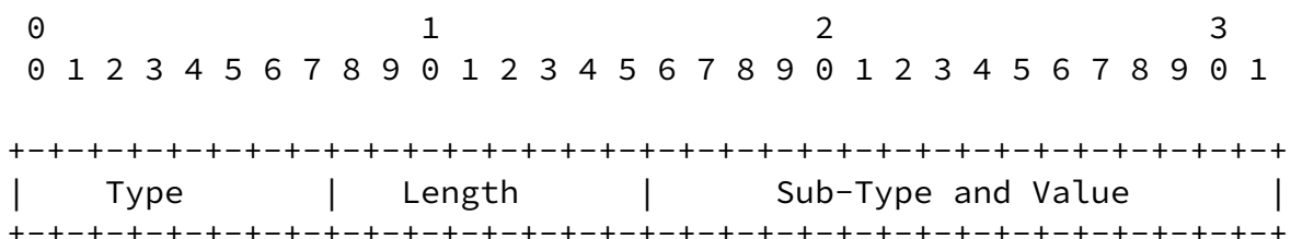
Figure 2: Link MSD Sub-TLV
