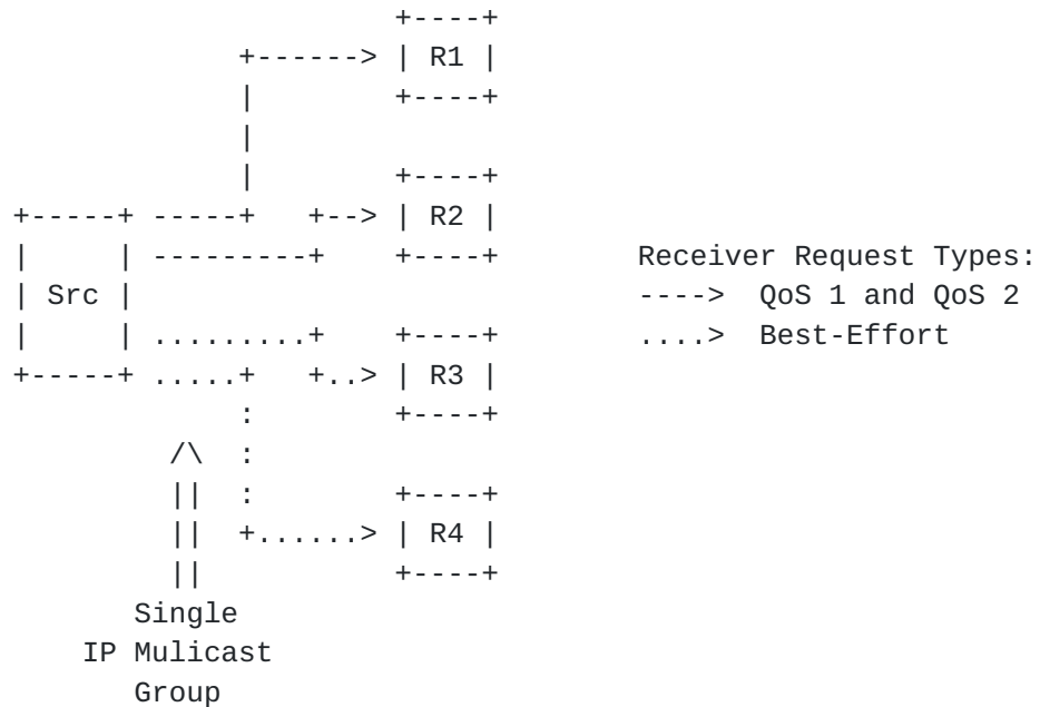
Figure 3: Types of Multicast Receivers
