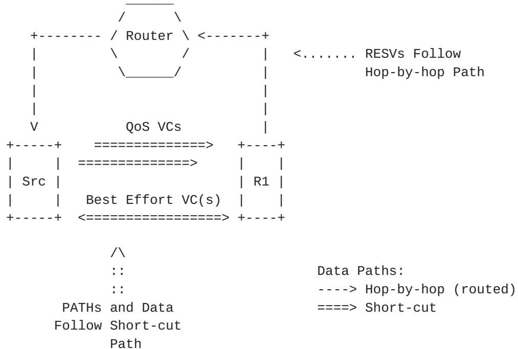
Figure 2: Asymmetric RSVP Message Forwarding With ATM Short-Cuts
