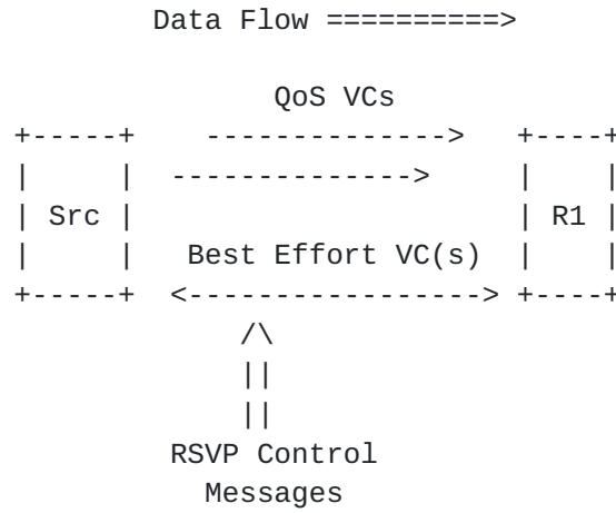
Figure 1: RSVP Control Message VC Usage
