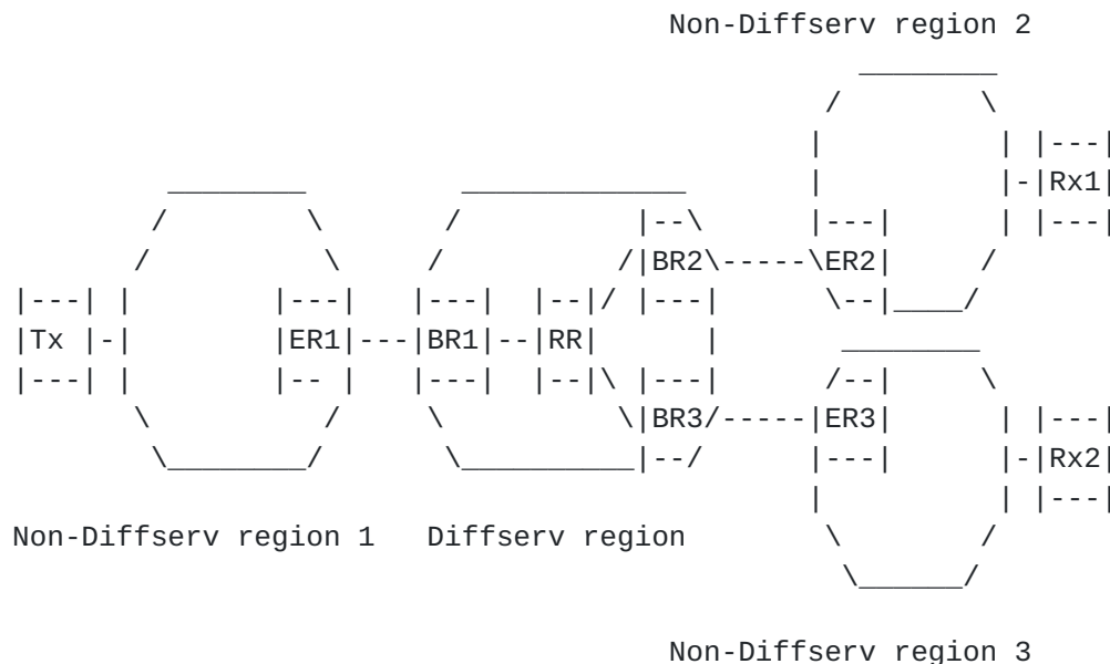
Figure 2: Sample Multicast Network Configuration
