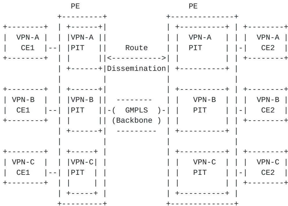
Figure 3 Basic Mode L1VPN Service
