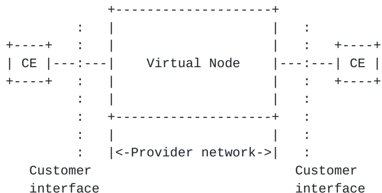
Figure 7.3: Virtual Node service model
