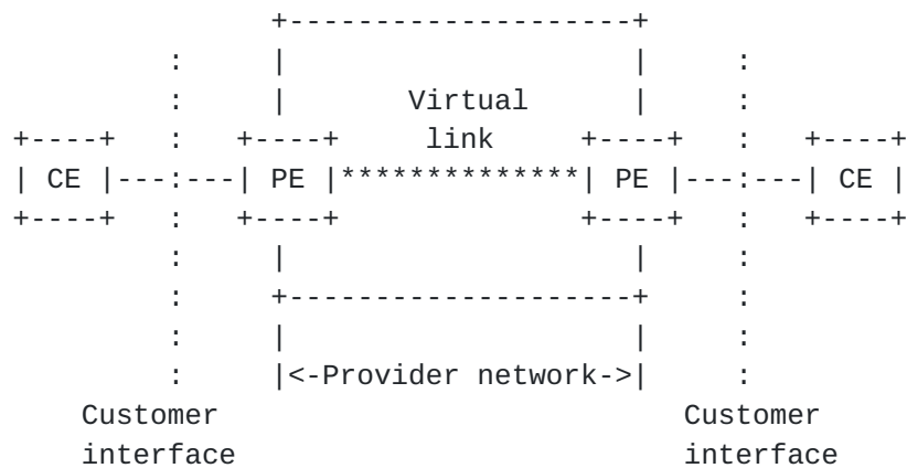
Figure 7.4: Virtual Link service model
