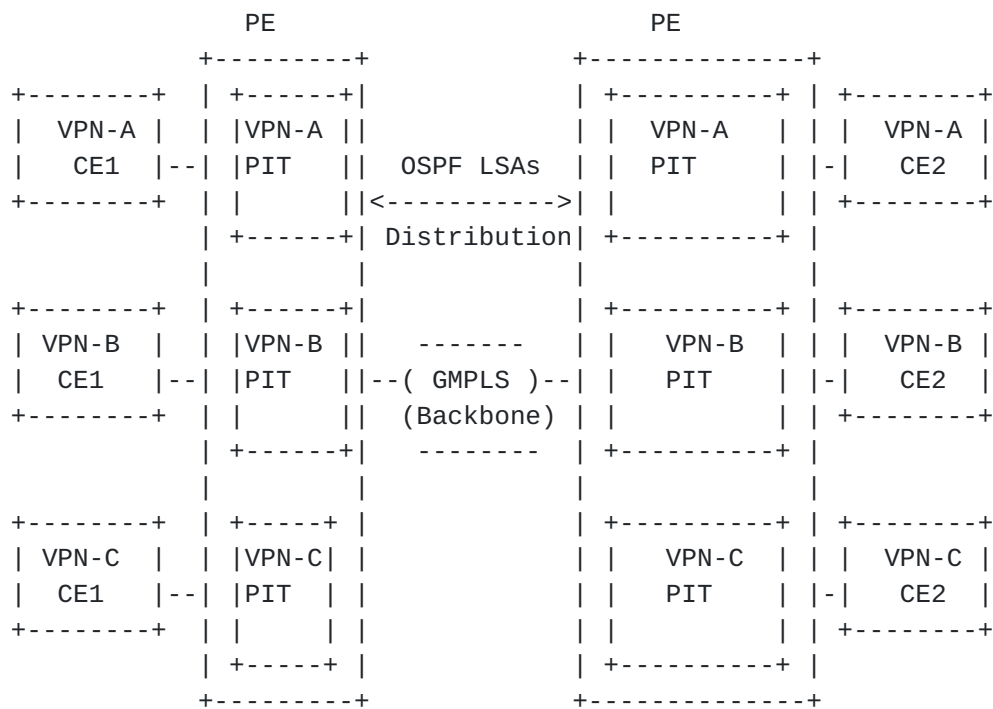
Figure 1: OSPF Auto-Discovery for L1VPNs
