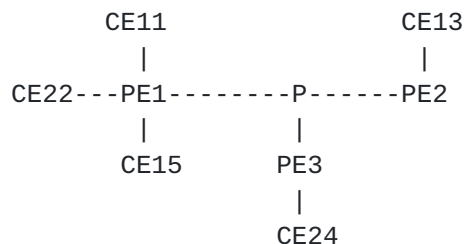
Figure 2: Single area configuration
