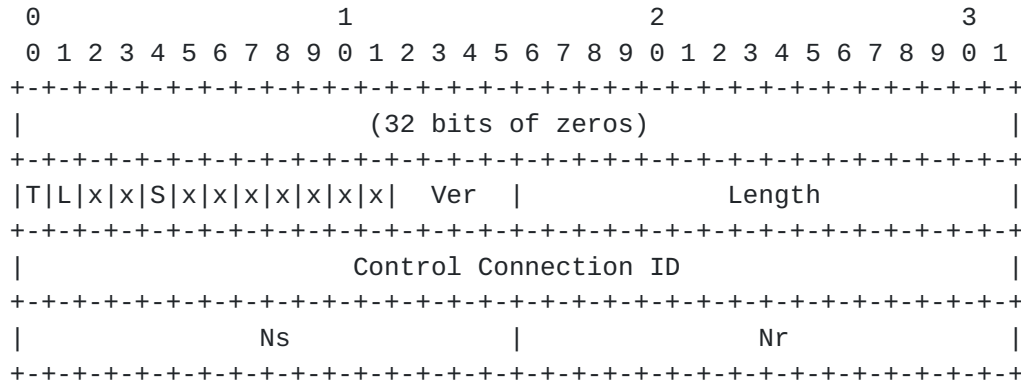
Figure 4.1.1.2: L2TPv3 Control Message Header Over IP
