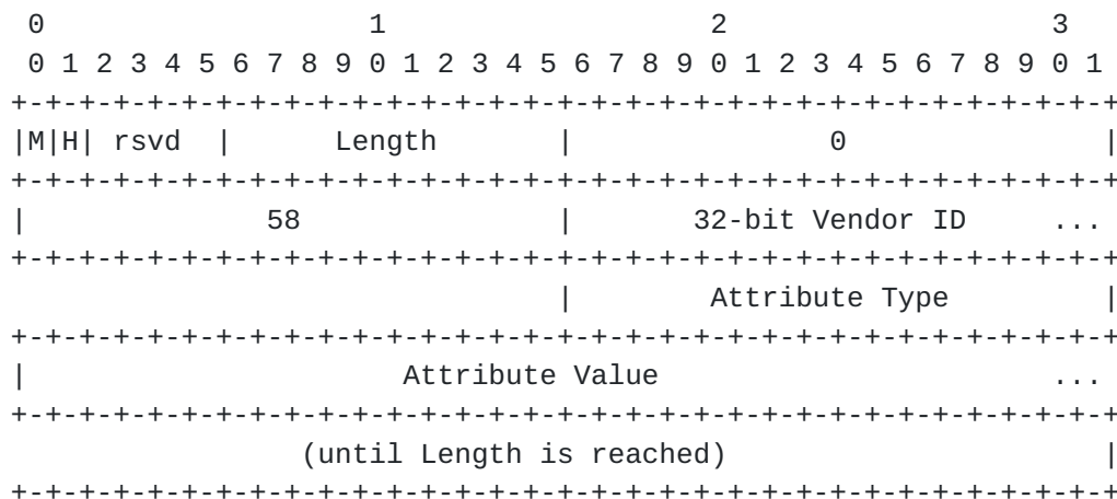
Figure 5.2: Extended Vendor ID AVP Format
