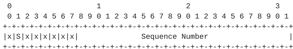
Figure 4.6: Default L2-Specific Sublayer Format
