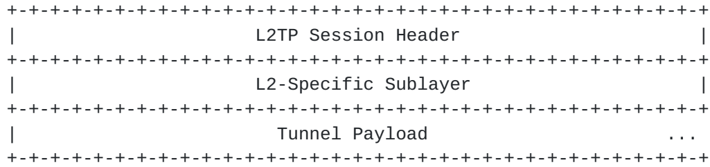
Figure 3.2.2: L2TP Data Message Header
