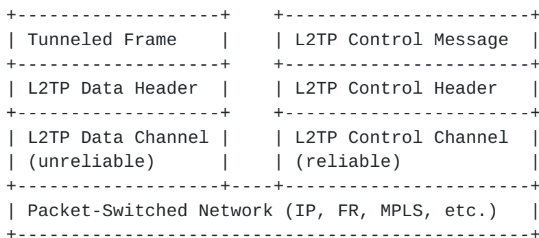
Figure 3.0: L2TPv3 Structure
