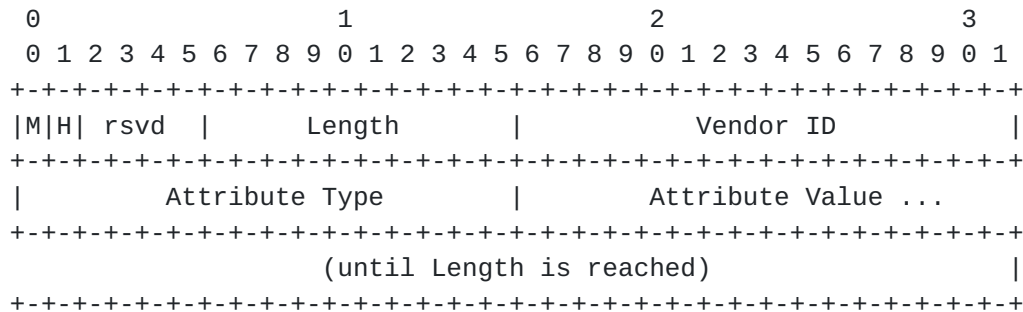
Figure 5.1: AVP Format
