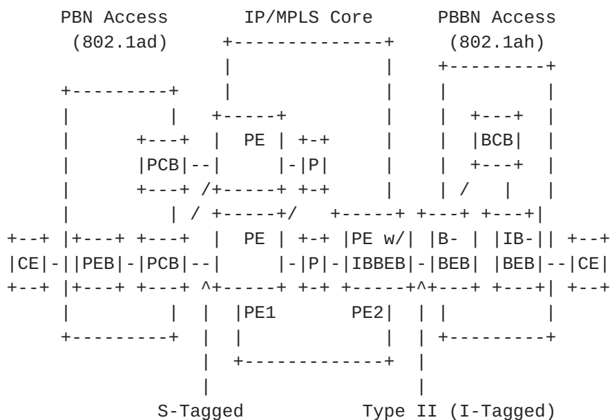
Figure 6: H-VPLS with Mixed PBN and PBBN Access: Regular PBN PE
