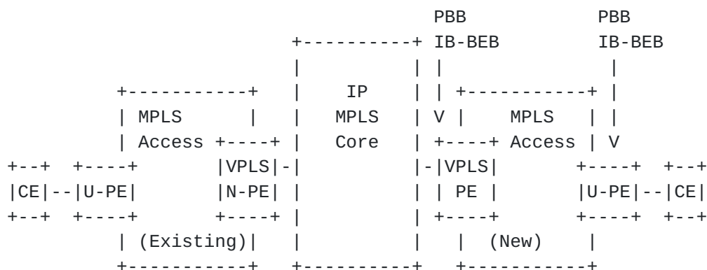
Figure 9: Migration with 802.1ad Service Frames over VPLS Core
