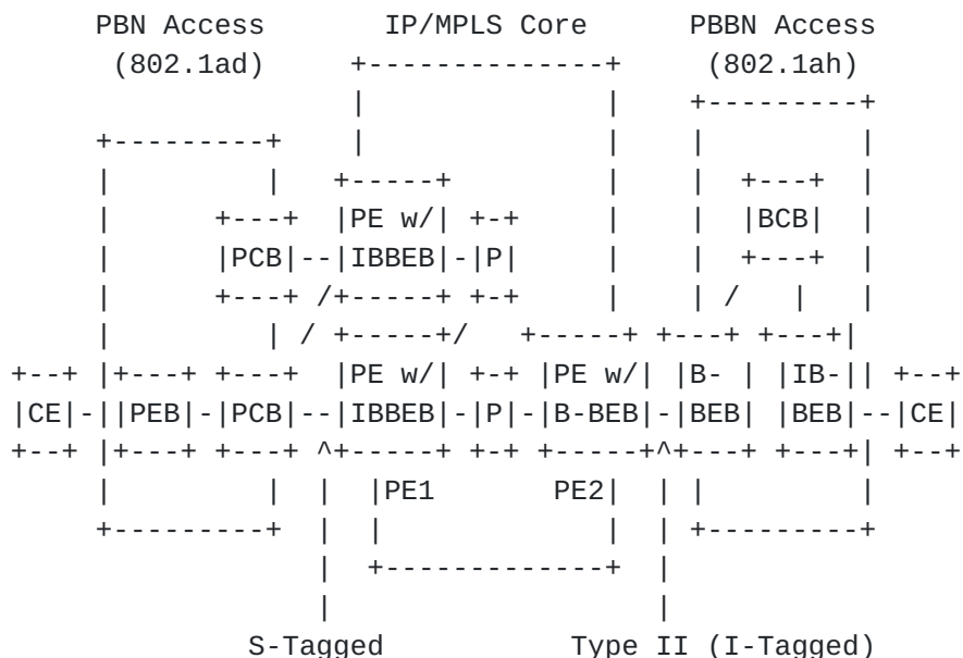
Figure 5: H-VPLS with Mixed PBN and PBBN Access: Modified PBN PE
