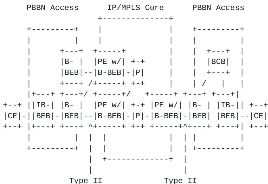
Figure 3: H-VPLS with PBBN Access &amp; Type II Service Interface
