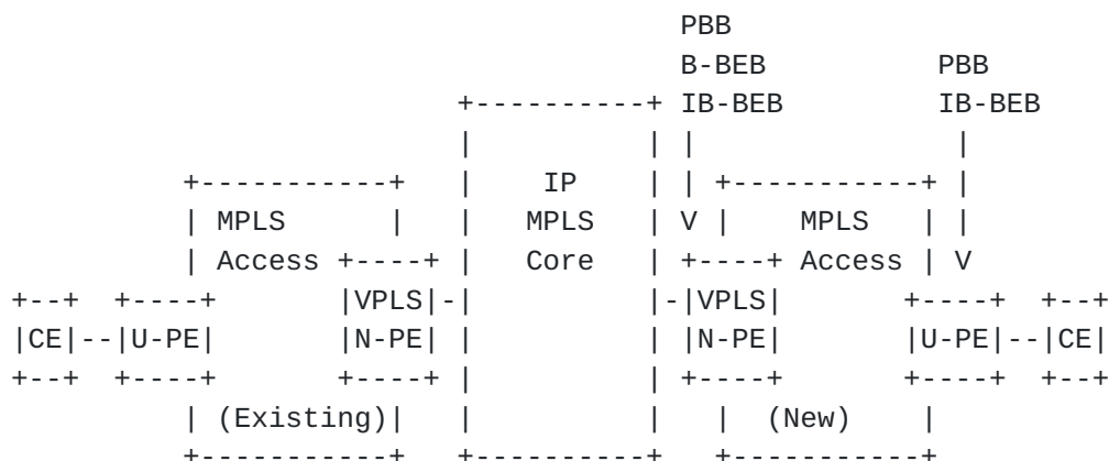
Figure 11: Migration with Mixed 802.1ad & PBB Service Frames over VPLS Core
