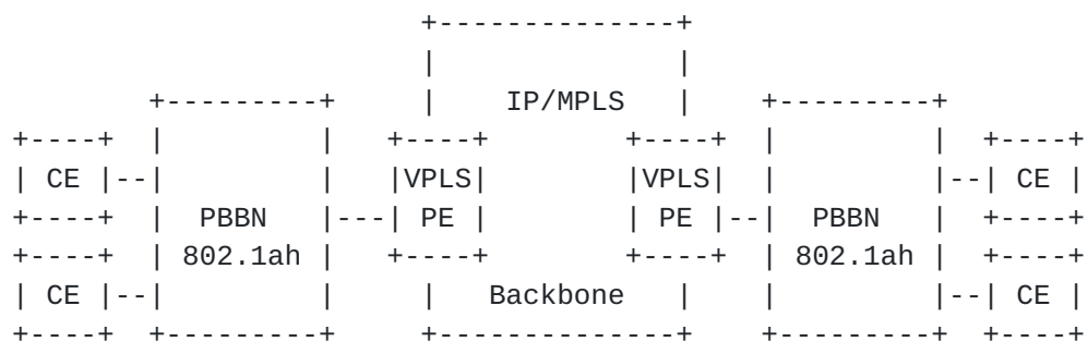
Figure 1: H-VPLS with PBBN Access
