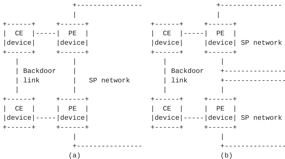
Figure 3 Backdoor Links Between CE Devices
