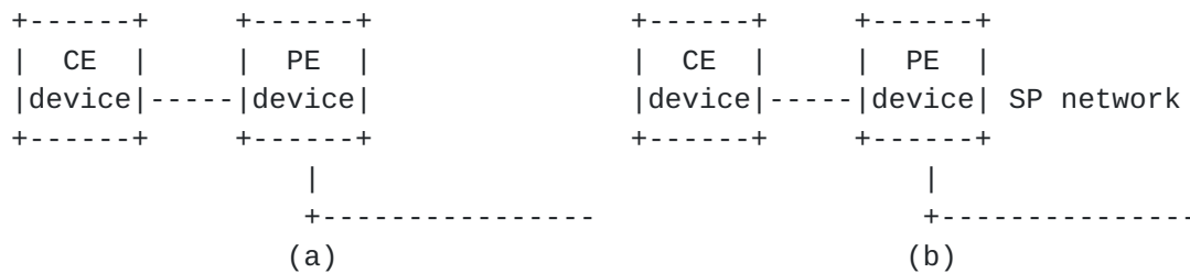
Figure 4 Combination of Dual-Homing and Backdoor Links for CE Devices
