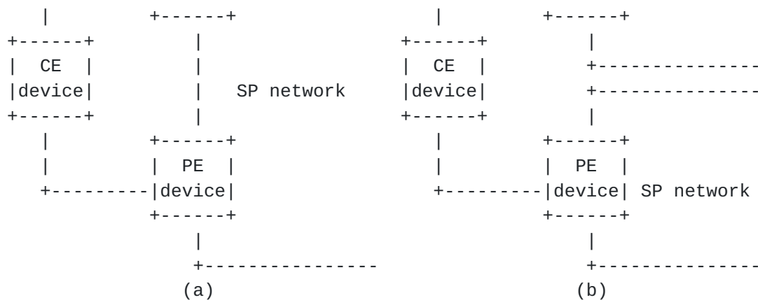
Figure 2 Dual-Homed Access of CE Devices
