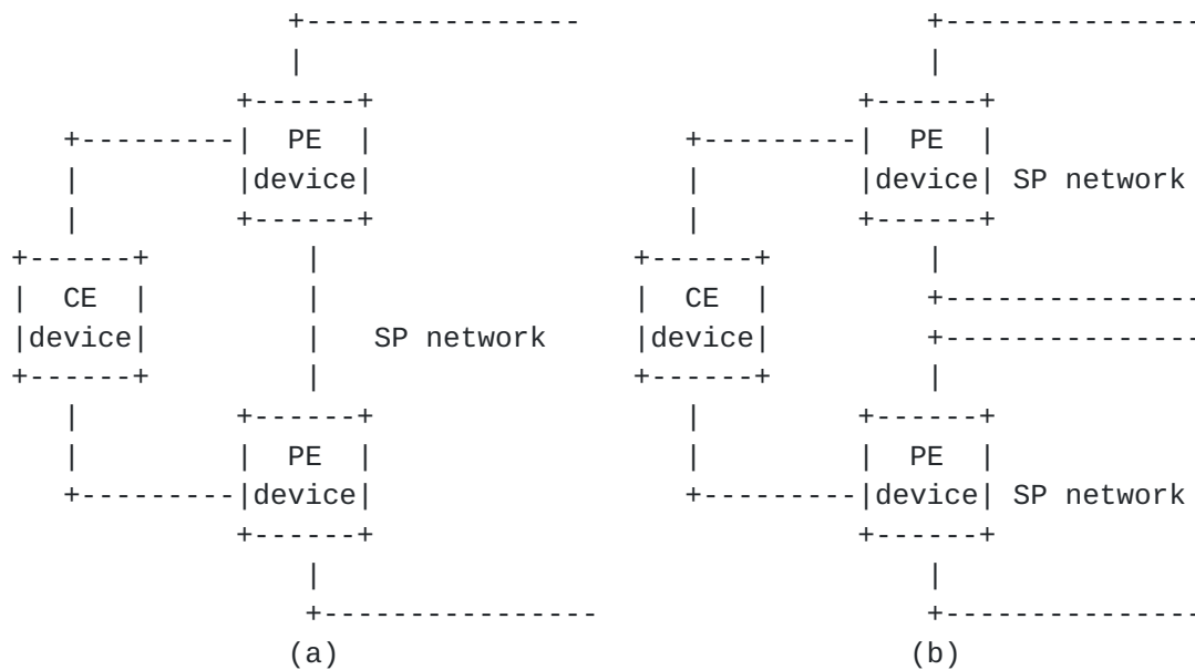
Figure 2 Dual-Homed Access of CE Devices
