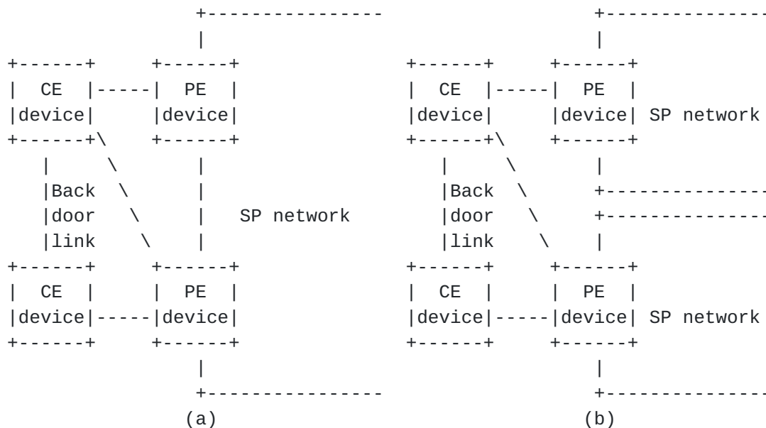
Figure 4 Combination of Dual-Homing and Backdoor Links for CE Devices
