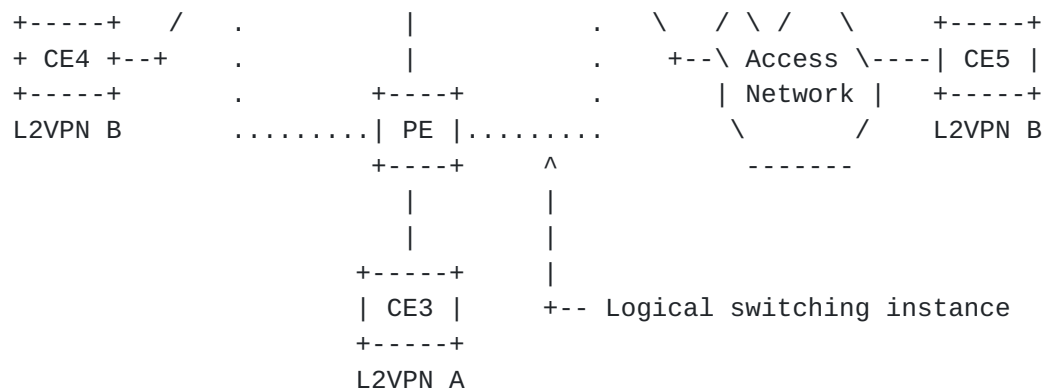
Figure 1 L2VPN Reference Model
