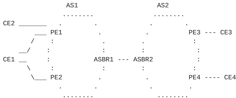
Figure 5 Inter-AS VPLS
