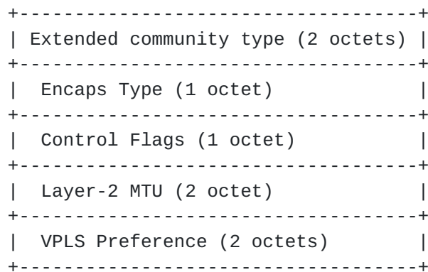
Figure 4 Layer 2 Info Extended Community
