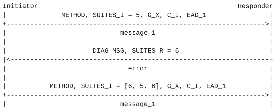
Figure 7: Example of Responder supporting suite 6 but not suite 5.
