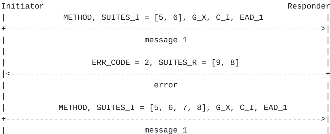
Figure 11: Example of an Initiator supporting suites 5, 6, 7, 8, and 9 in decreasing order of preference, and a Responder supporting suites 8 and 9 but not 5, 6 or 7. The Responder rejects the first message_1 with an error indicating support for suites 8 and 9 (in any order). The Initiator also supports suites 8 and 9, and prefers suite 8, so therefore selects suite 8 in the second message_1. The initiator prepends in SUITES_I the selected suite 8 with the more preferred suites in order of preference, in this case suites 5, 6 and 7, to mitigate a potential attack on the cipher suite negotiation.
