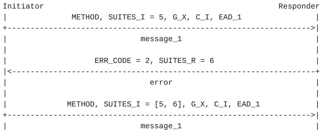
Figure 10: Example of an Initiator supporting suites 5, 6, 7, 8, and 9 in decreasing order of preference, and a Responder supporting suite 6 but not suite 5. The Responder rejects the first message_1 with an error indicating support for suite 6. The Initiator also supports suite 6, and therefore selects suite 6 in the second message_1. The initiator prepends in SUITES_I the selected suite 6 with the more preferred suites, in this case suite 5, to mitigate a potential attack on the cipher suite negotiation.
