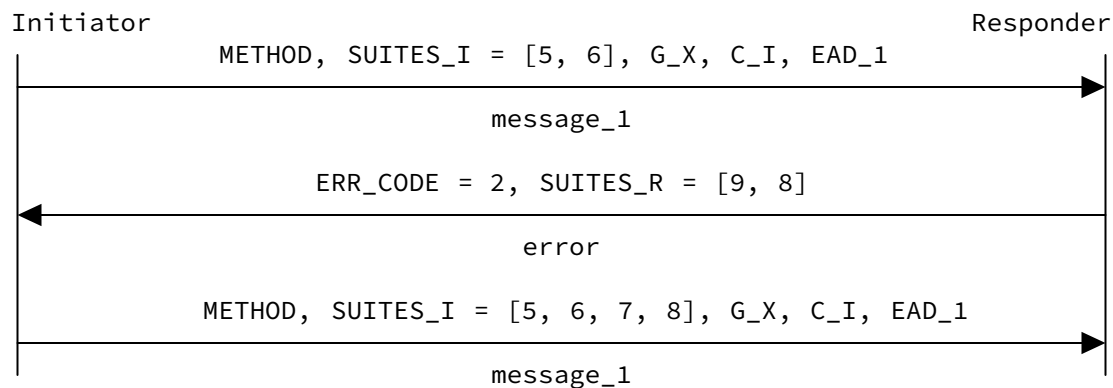
Figure 12: Cipher suite negotiation example 2.
