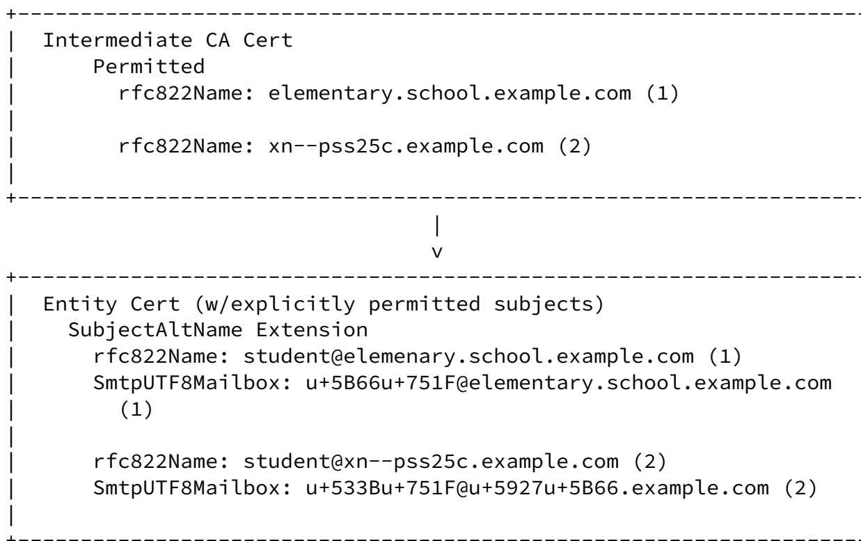
Name constraints with Smtputf8Name and rfc822Name
