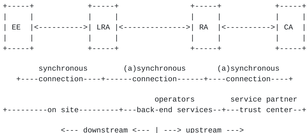
Figure 1: Certificate Management Architecture Example
