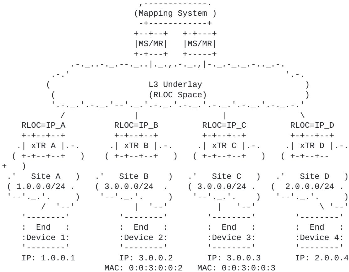
Figure 1: Reference System Architecture with unified L2 and L3 overlays
