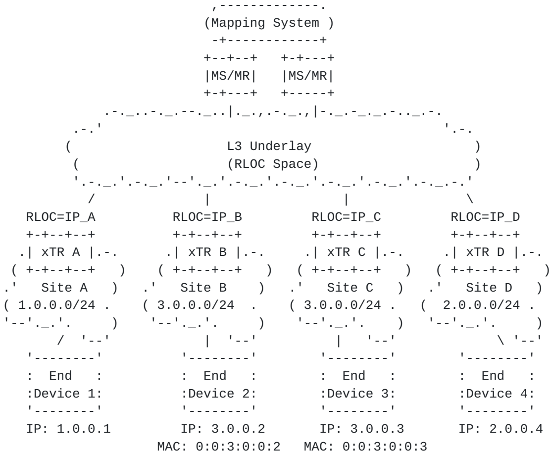
Figure 1: Reference System Architecture with unified L2 and L3 overlays
