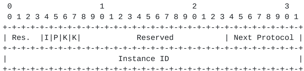
Figure 2: LISP-GPE Header
