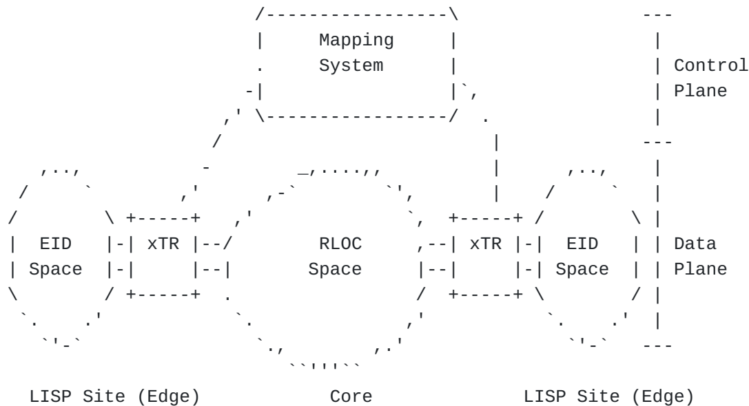
Figure 1: A schema of the LISP Architecture.
