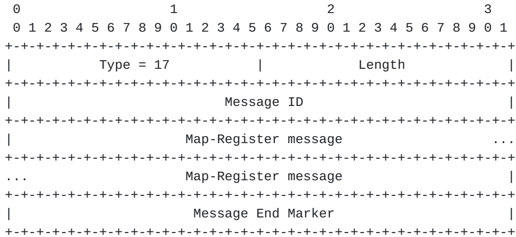
Registration message format
