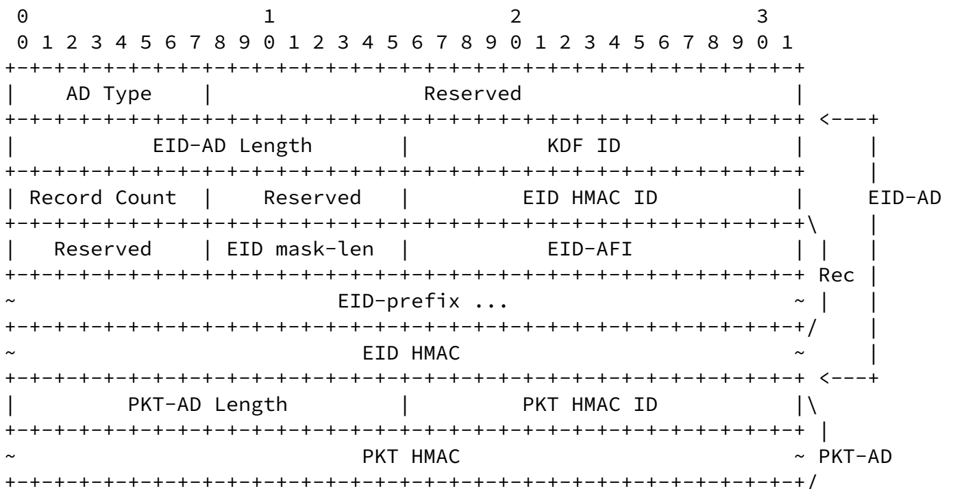
LISP-SEC Map-Reply Authentication Data
