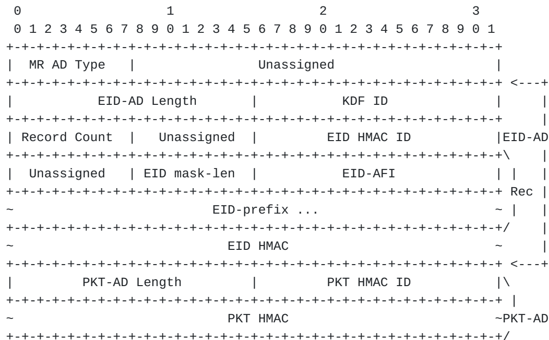
Figure 2: LISP-SEC Map-Reply Authentication Data
