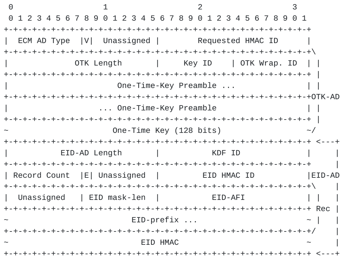
Figure 1: LISP-SEC ECM Authentication Data
