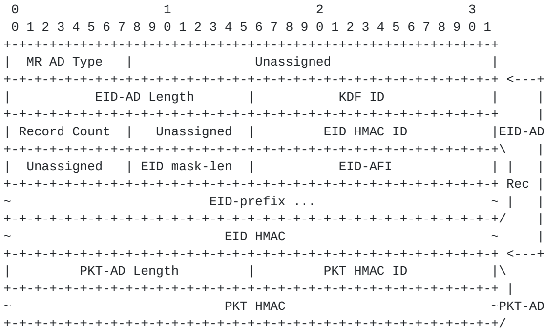
Figure 2: LISP-SEC Map-Reply Authentication Data
