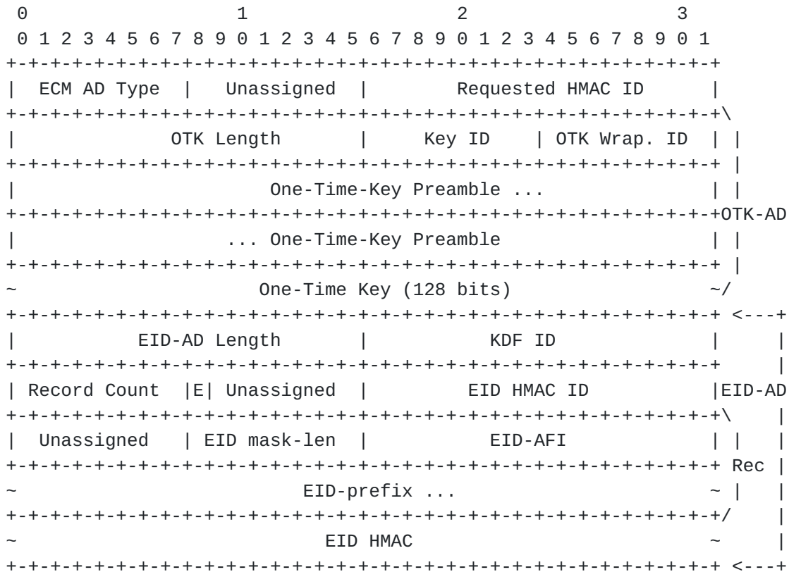
Figure 1: LISP-SEC ECM Authentication Data
