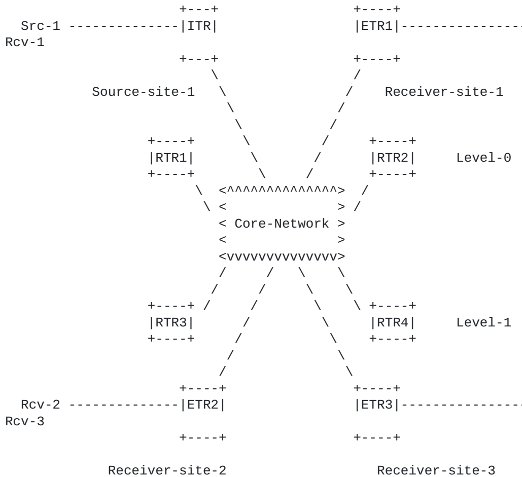
Figure 2: LISP-RE Reference Model
