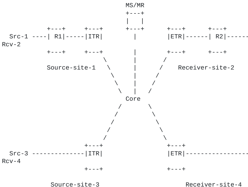
Figure 1: LISP Multicast Generic Reference Model
