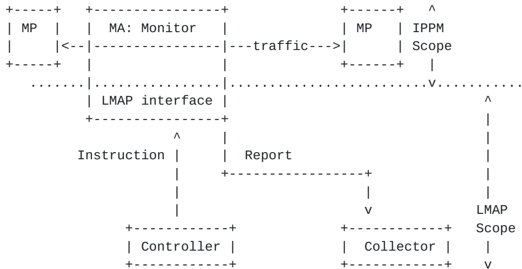
Figure A4: Schematic of LMAP-based measurement system, with a Measurement Agent monitoring traffic
