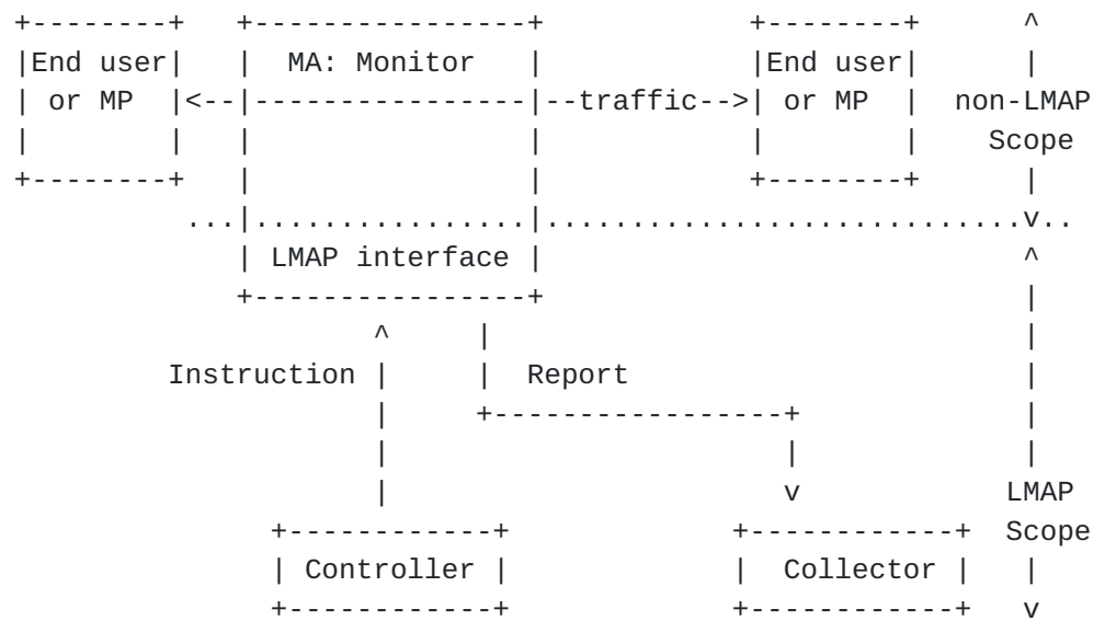
Figure A4: Schematic of LMAP-based Measurement System, with a Measurement Agent monitoring traffic
