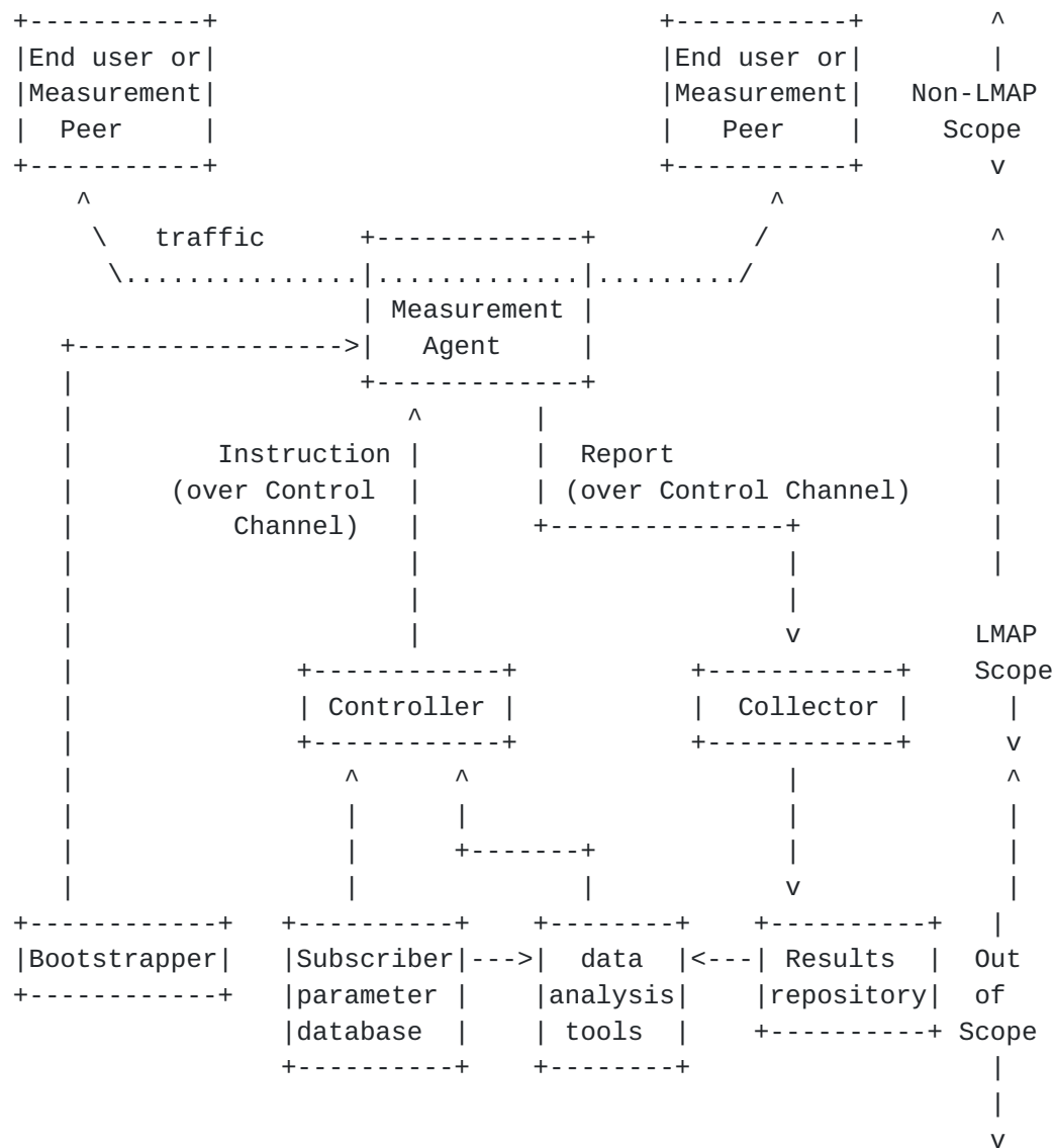
Figure 1: Schematic of main elements of an LMAP-based Measurement System (showing the elements in and out of the scope of initial LMAP work)
