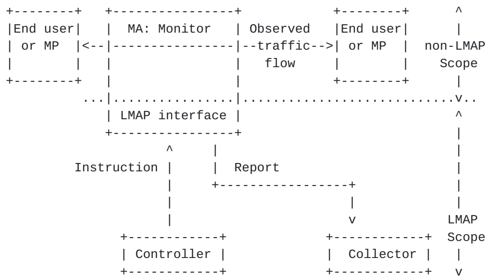
Schematic of LMAP-based Measurement System, with a Measurement Agent monitoring traffic
