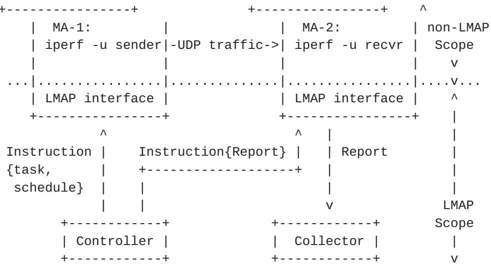
Schematic of LMAP-based Measurement System, with two Measurement Agents cooperating to measure UDP traffic
