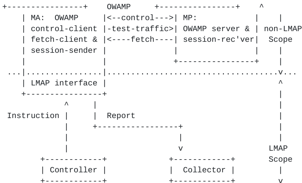
Schematic of LMAP-based Measurement System, with OWAMP server as Measurement Peer
