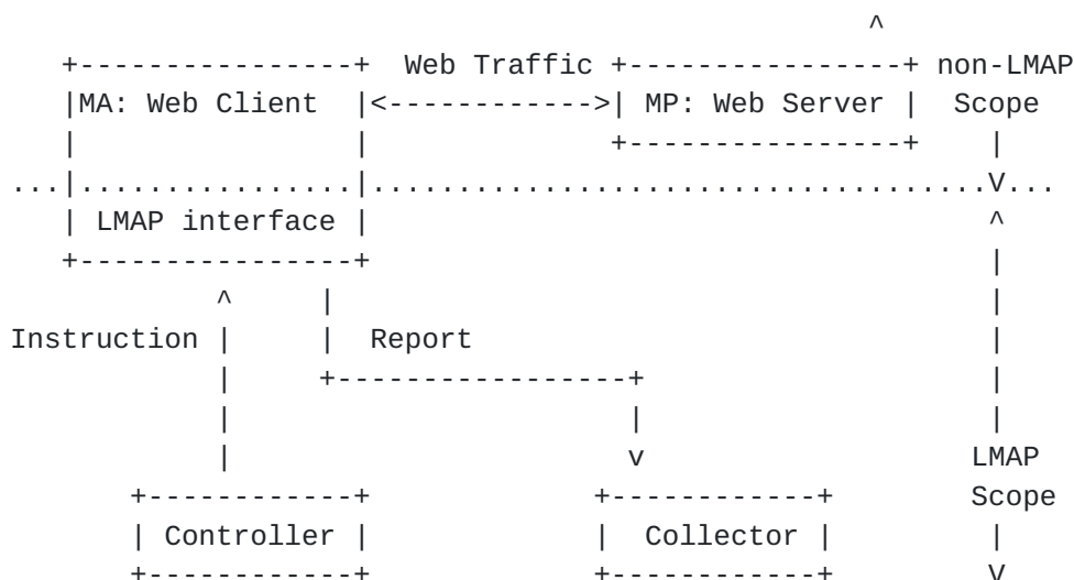
Schematic of LMAP-based Measurement System, with Web server as Measurement Peer
