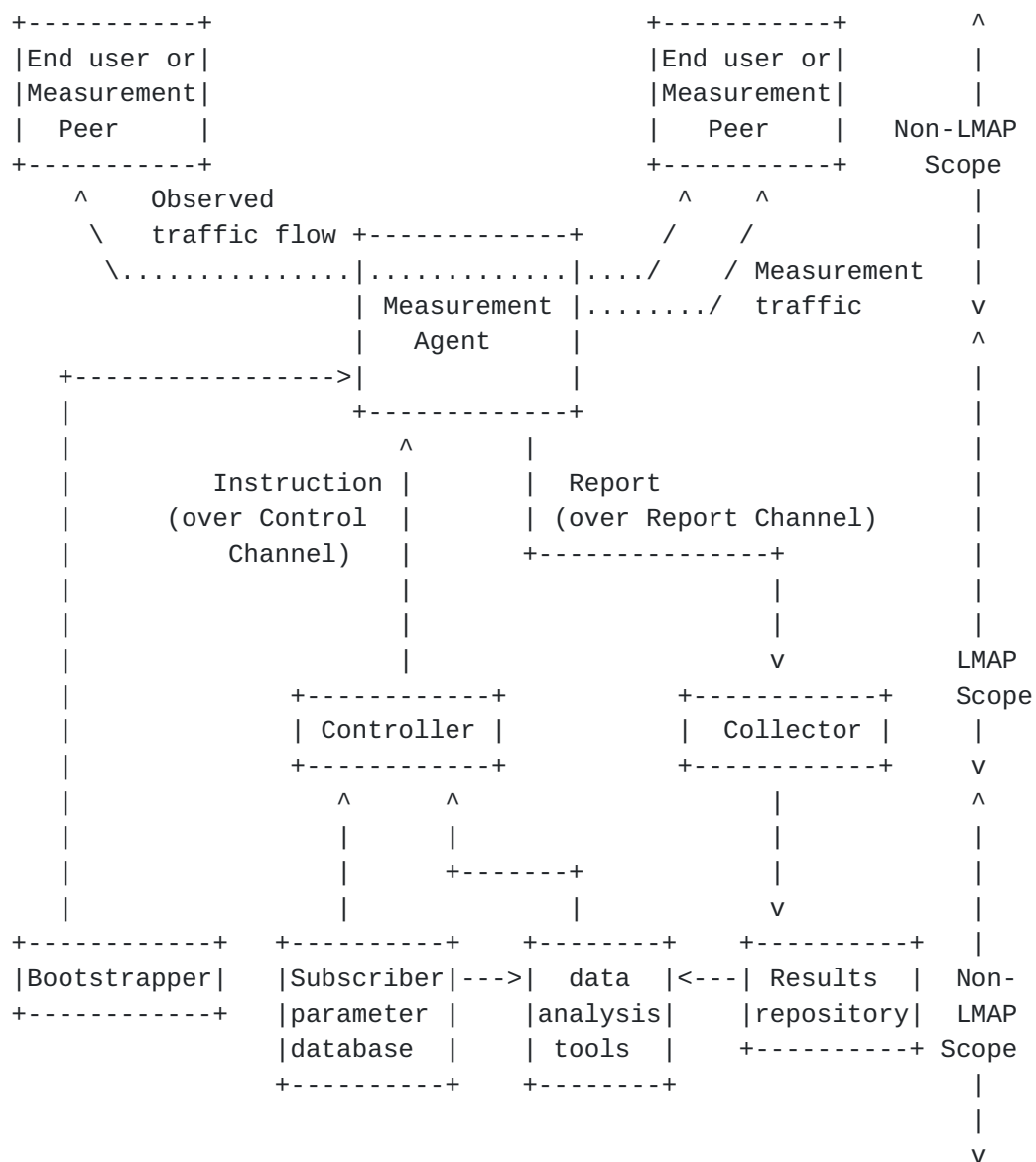
Schematic of main elements of an LMAP-based Measurement System (showing the elements in and out of the scope of initial LMAP work)
