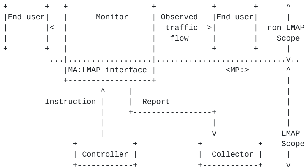
Schematic of LMAP-based Measurement System, with a Measurement Agent monitoring traffic
