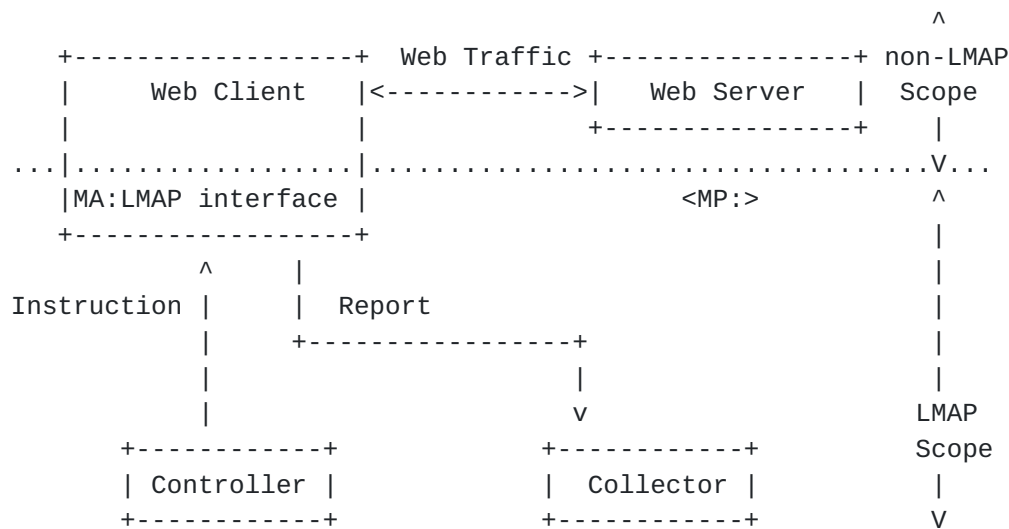
Schematic of LMAP-based Measurement System, with Web server as Measurement Peer
