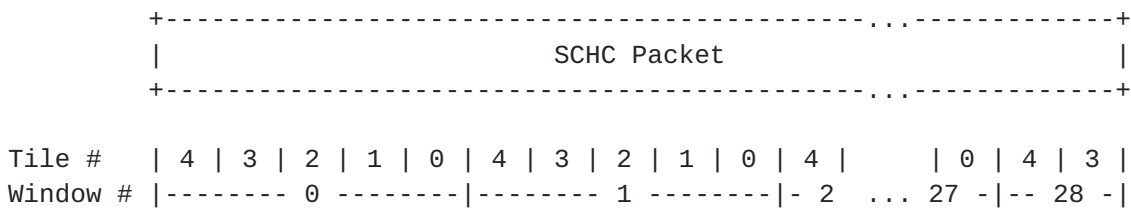
Figure 11: a SCHC Packet fragmented in tiles grouped in 29 windows, with WINDOW_SIZE = 5
