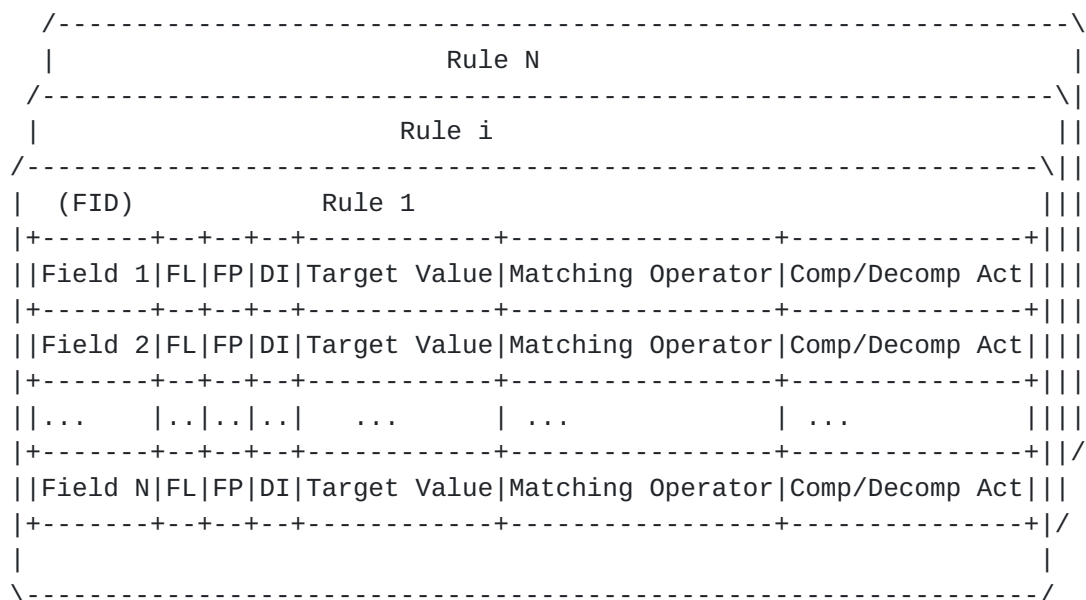
Figure 6: A Compression/Decompression Context
