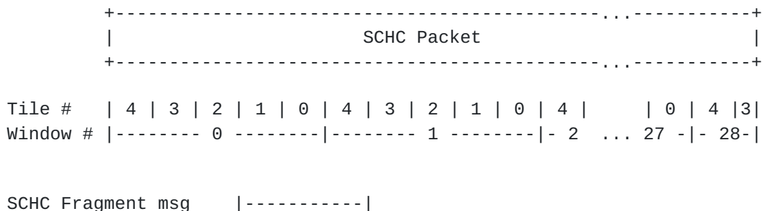
Figure 23: a SCHC Packet fragmented in tiles, ACK-on-Error mode
