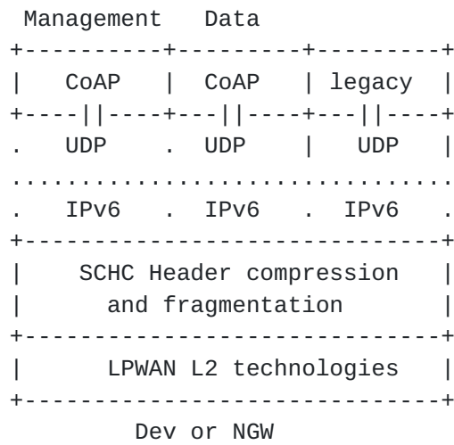
Figure 25: Simplified Protocol Stack for LP-WAN
