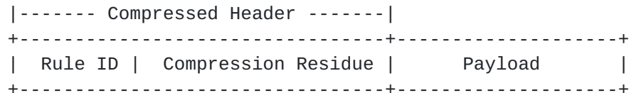
Figure 4: SCHC Packet
