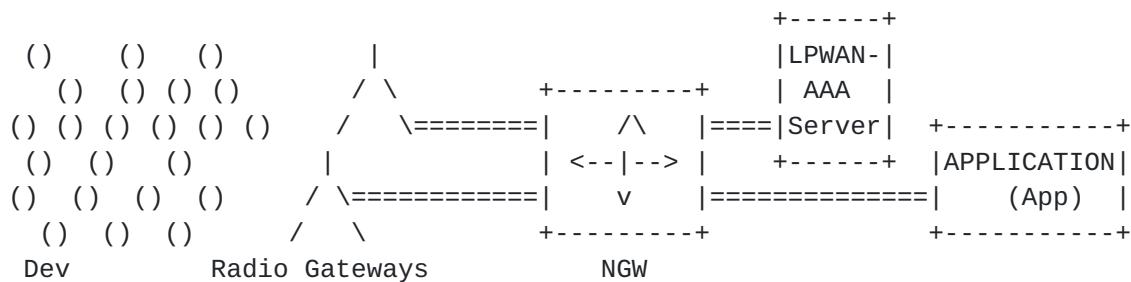
Figure 9: LPWAN Architecture
