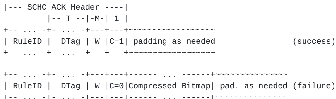
Figure 4: Acknowledgment fragment header for RFC8724
