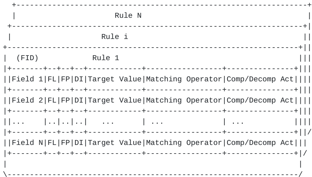
Figure 1: Compression Decompression Context
