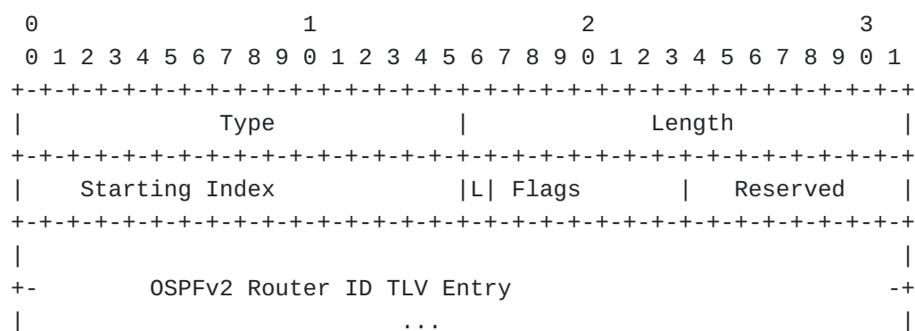
Figure 4: OSPFv2 Area Router IDs TLV
