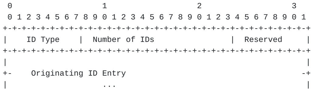
Figure 6: OSPFv3 Router ID TLV Entry
