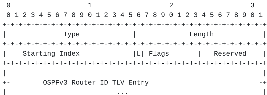
Figure 5: OSPFv3 Area Router IDs TLV
