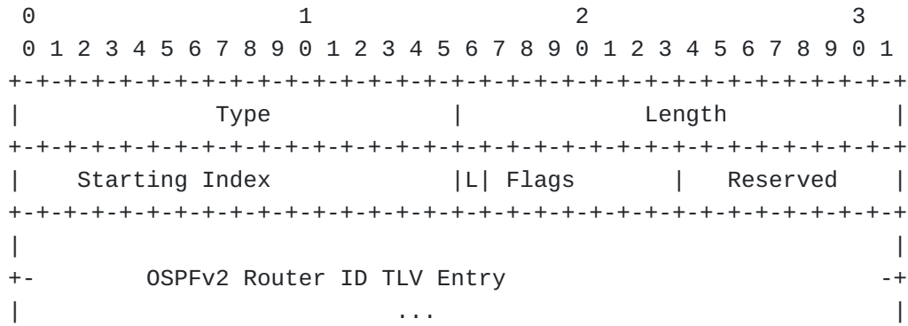
Figure 3: OSPFv2 Area Router IDs TLV
