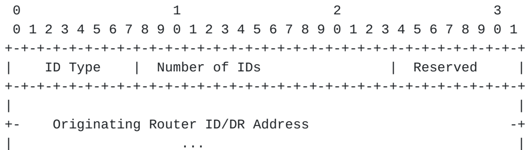
Figure 4: OSPFv2 Router IDs TLV Entry
