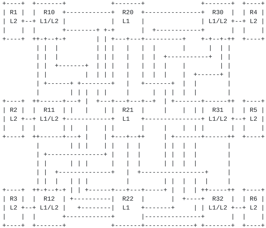
Figure 1: Example topology
