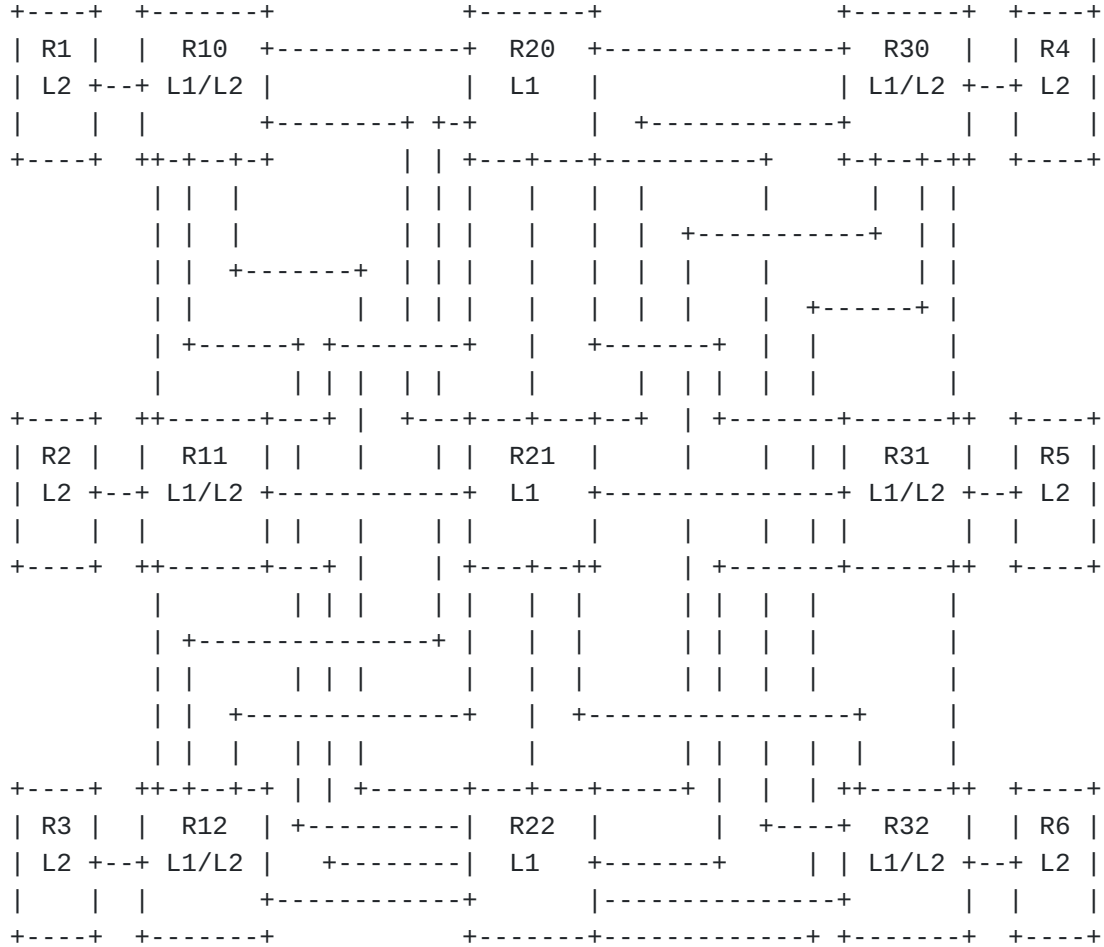
Figure 1: Example topology
