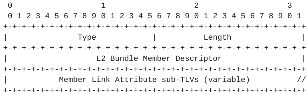
Figure 1: L2 Bundle Member Attributes sub-TLV Format
