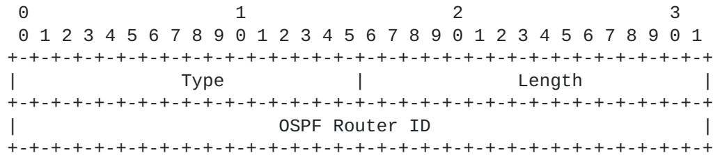
Figure 1: Prefix Source Router-ID Sub-TLV Format
