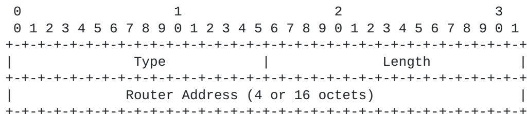
Figure 2: Prefix Originator Sub-TLV Format
