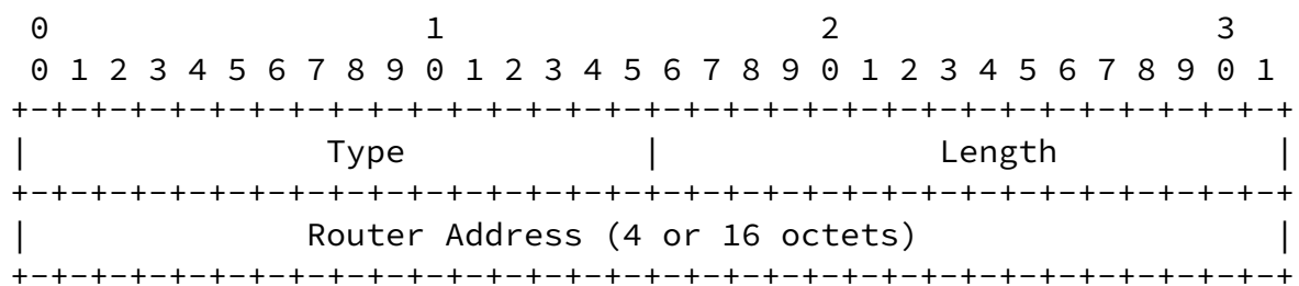
Figure 2: Prefix Source Router Address Sub-TLV Format
