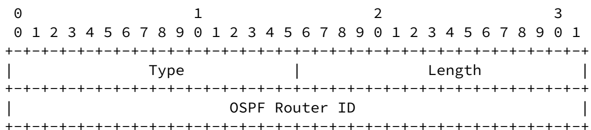
Figure 1: Prefix Source OSPF Router-ID Sub-TLV Format
