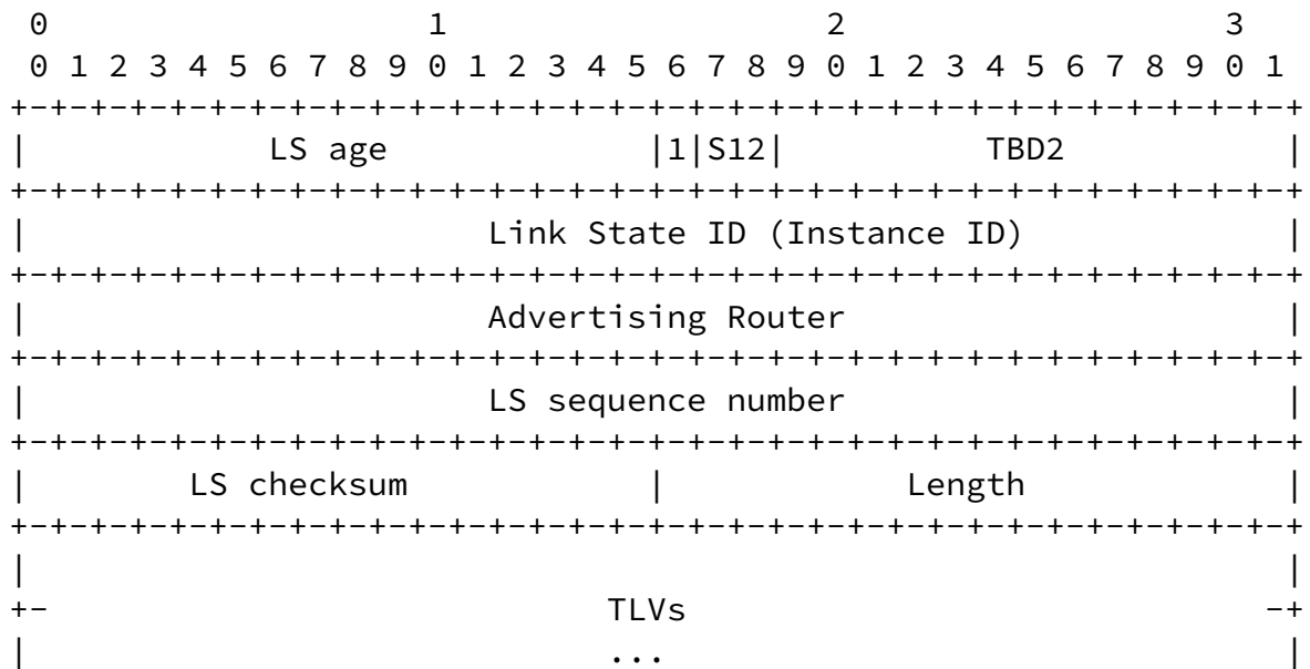
Figure 3: OSPFv3 Transport Instance Information LSA
