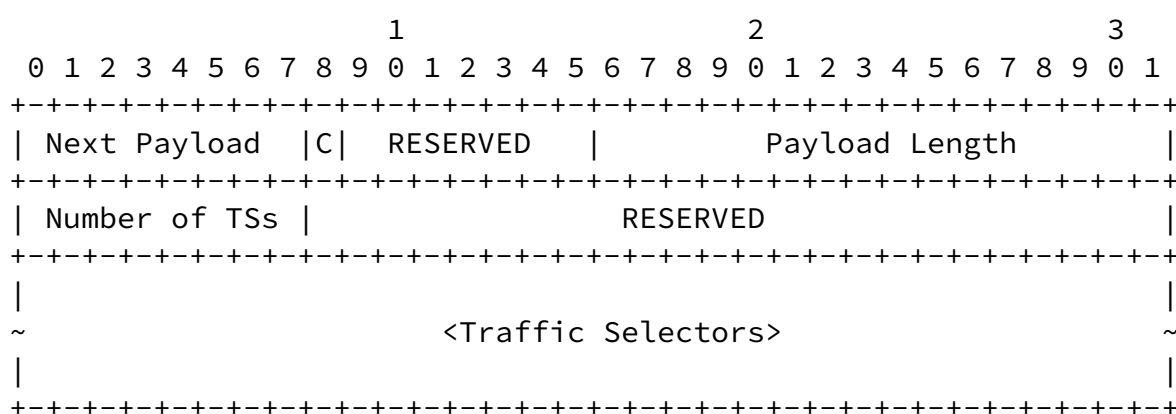
Figure 14: Traffic Selectors Payload Format
