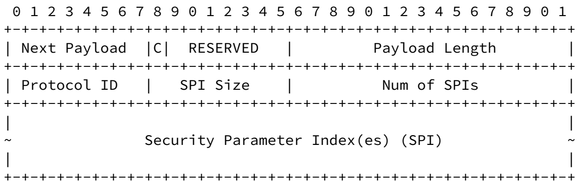
Figure 17: Delete Payload Format
